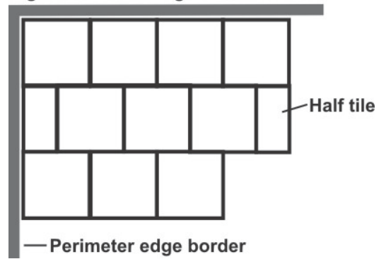
Figure C - Installing within new border
